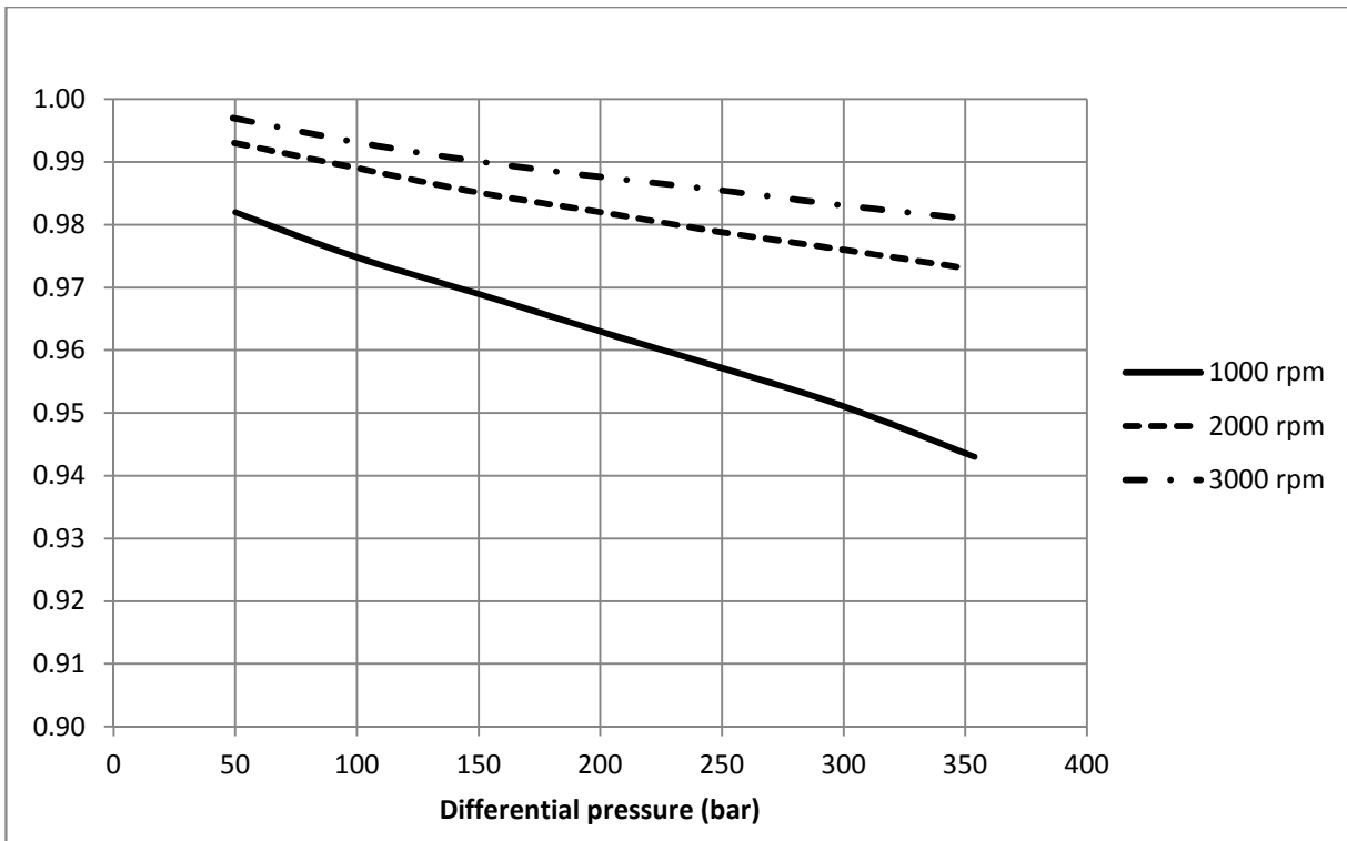
SCM 012 Volumetric efficiency
