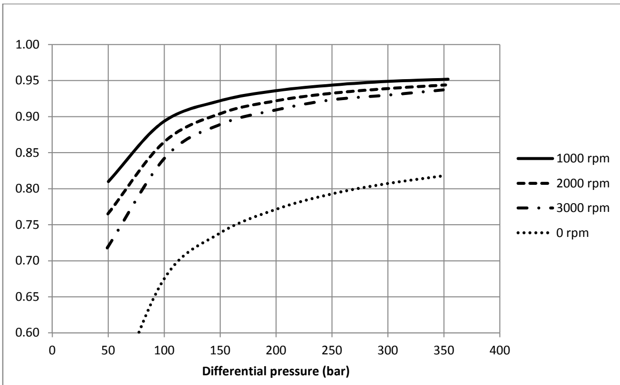
SCM 012 Hydraulic-mechanical efficiency
