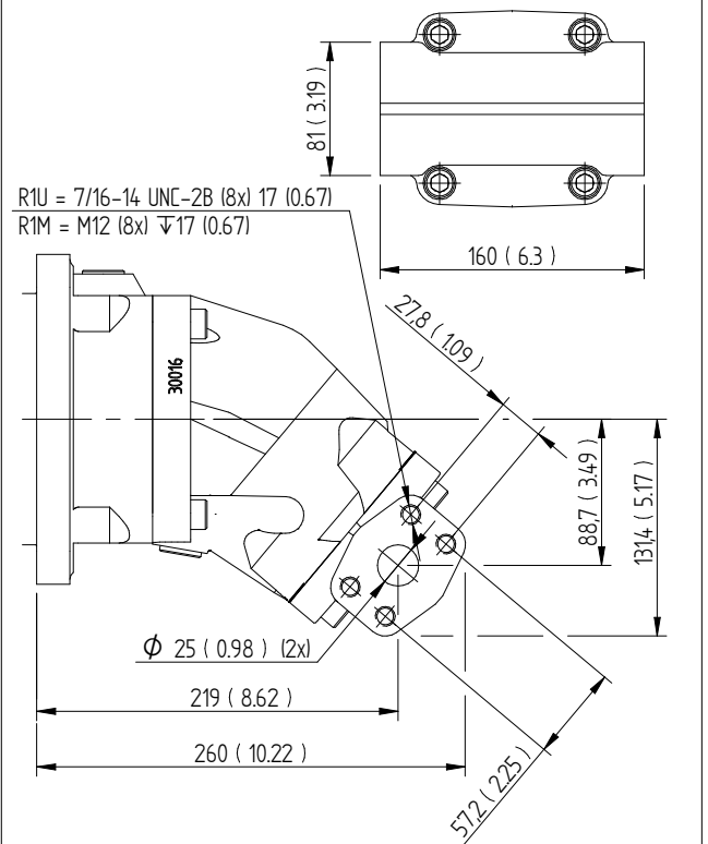
R1U/R1M 084-108 SAE J518, 1 in
