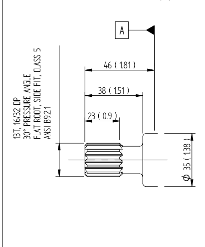
B13 SAE J744, ID. Code: 22-4 (B)
