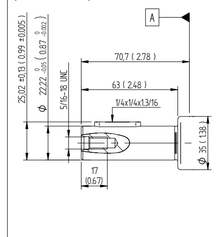
B22 SAE J744, ID. Code: 22-1 (B) (010-017 ONLY)
