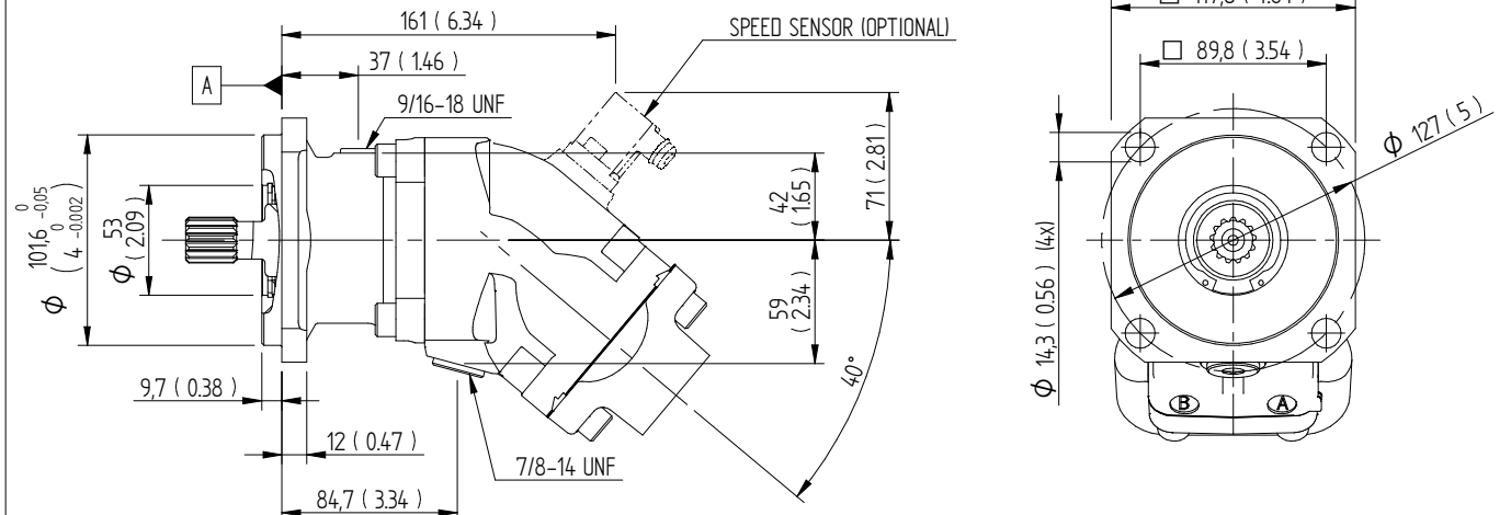
SB4 SAE J744, ID. Code: 101-4 (B)
